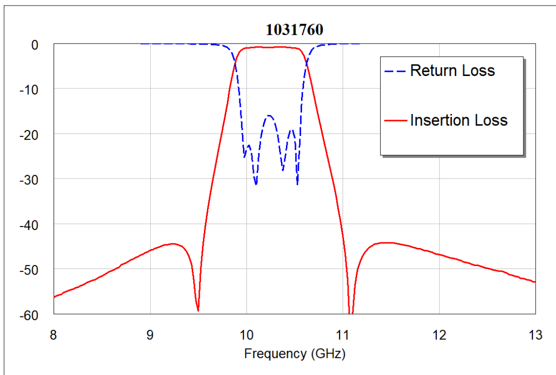
Figure 1: RF performance
