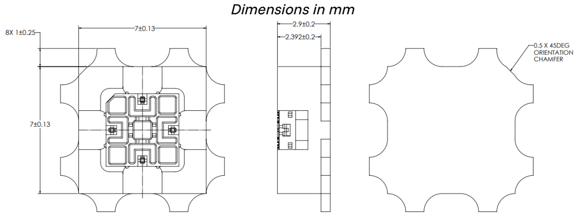
Figure 3: 2D Mechanical Drawing
