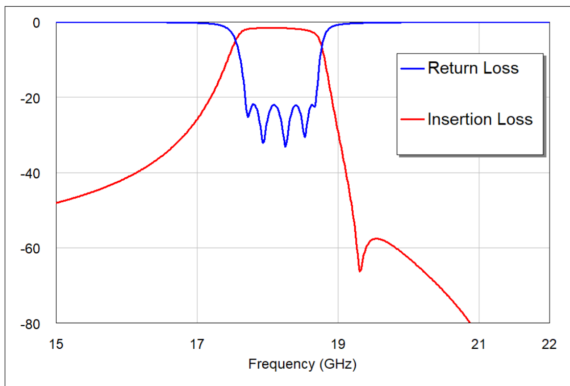
Figure 1: RF performance
