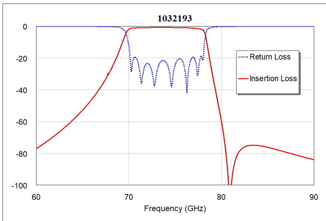
Figure 1: RF performance
