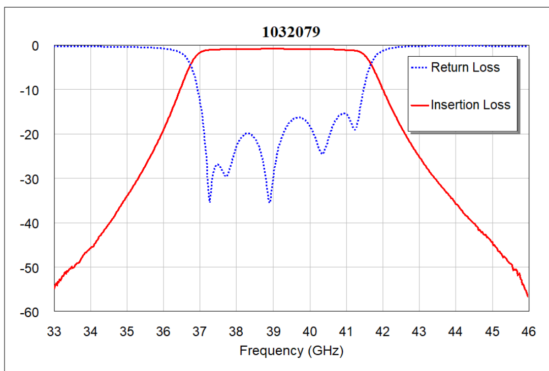
Figure 1: RF performance
