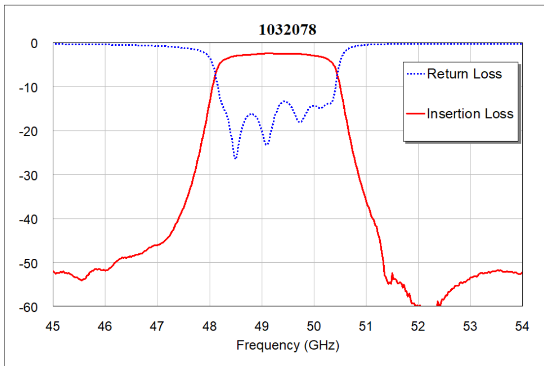
Figure 1: RF performance
