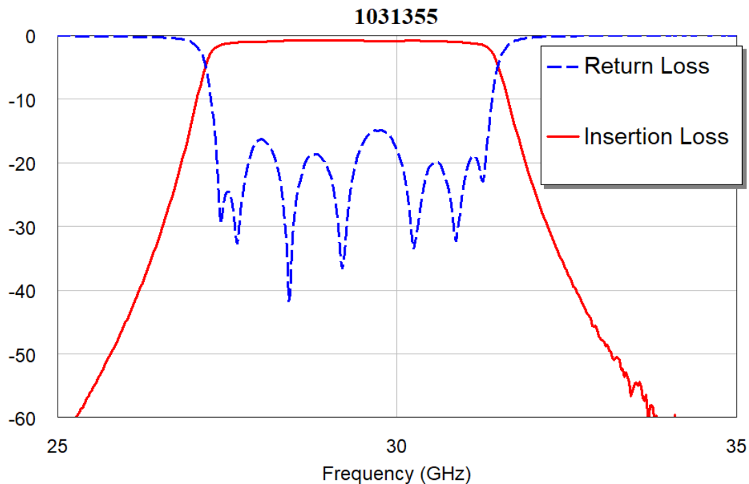
Figure 1: RF performance
