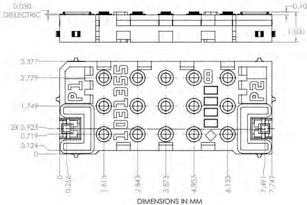
Figure 3: 2D Mechanical Drawing
