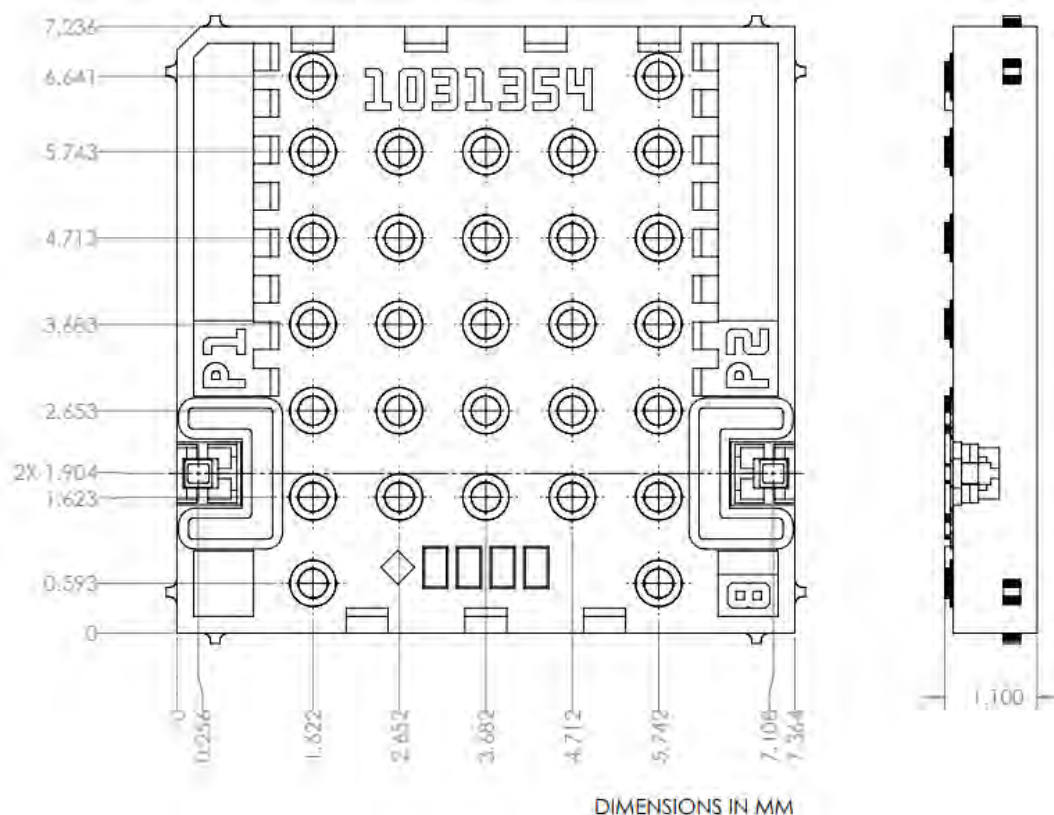
Figure 3: 2D Mechanical Drawing
